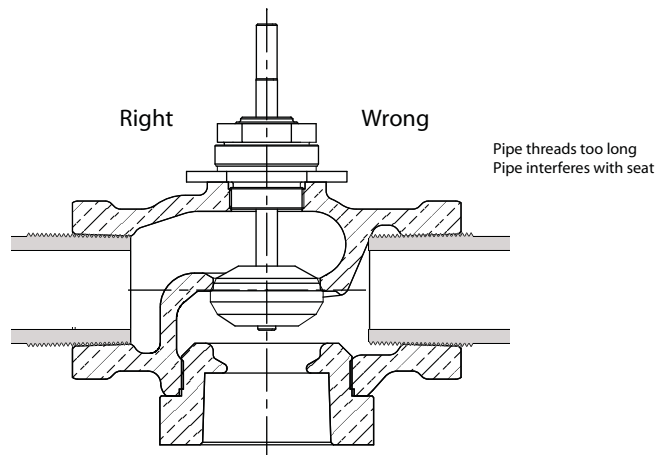
Figure-3 Normal Thread Engagement.
