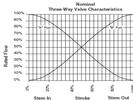
Figure-1 Typical Flow Characteristics.
