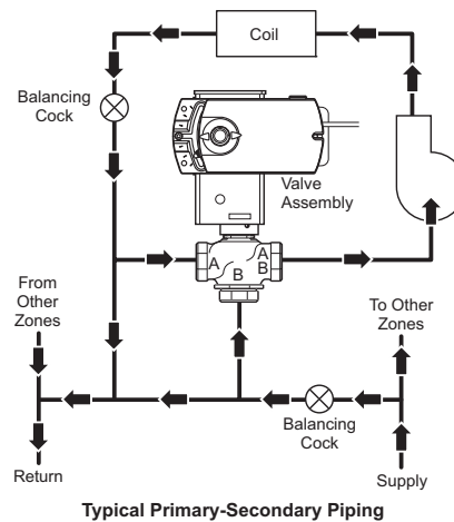
Figure-7 Typical Primary-Secondary Piping.
