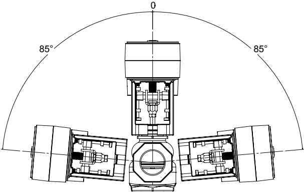
IP51 and NEMA Type 2 Allowable Mounting Orientation
