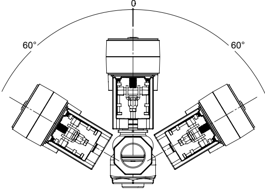
IP53 and NEMA Type 2 Allowable Mounting Orientation
