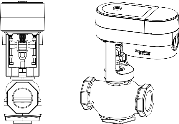
End View Side View MG350V Installed on a VB-7000 Globe Valve
